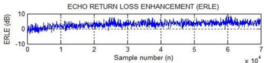
Figure (9) Echo Return Loss Enhancement (ERLE) [dB] (with \mu=0.05 and N=32 ).
