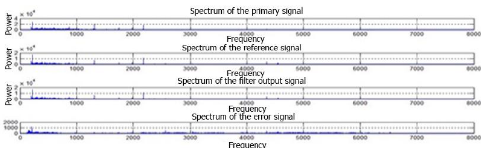
Figure (6) the frequency spectrum primary, the reference, the filter output and the error signals ( \mu=0.05 , N=32 ).
