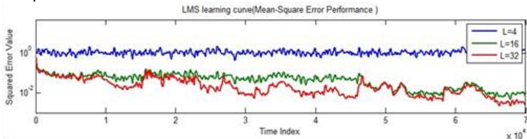
Figure (3) Behavior of NLMS algorithm for different filter length and with a step-size parameter \mu=0.05
