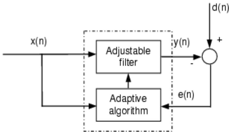
Figure (1) Block Diagram of General Adaptive Filter
