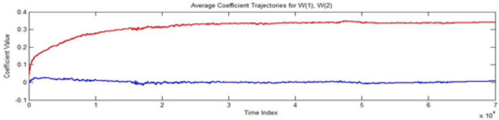
Figure (7) The Average Coefficient Trajectories for W (1), W (2) and the learning curve (with \mu=0.05 and N=32 ).
