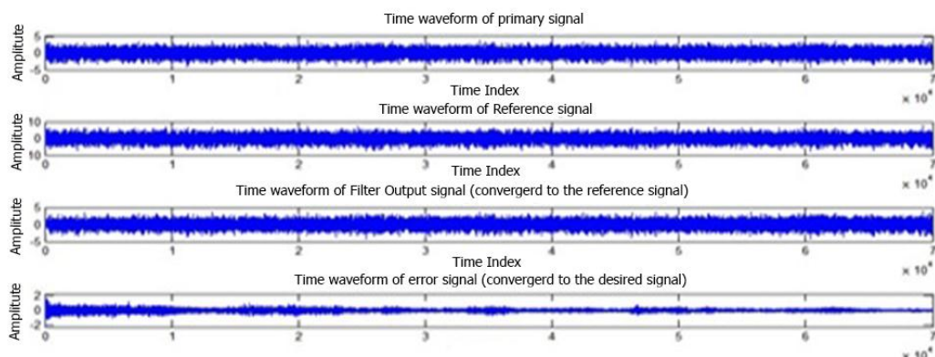
Figure (5) the primary, the reference, the filter output and the error signals (with \mu=0.05 and N=32 ).
