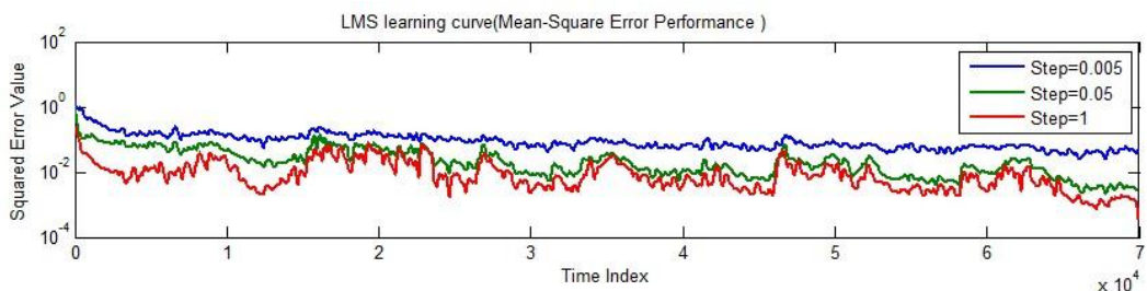
Figure (4) Evolution of the Mean Square Error for different values of the step size ( \mu ) (L=32).
