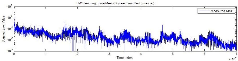
Figure (8) the learning curve (with \mu=0.05 and N=32 ).
